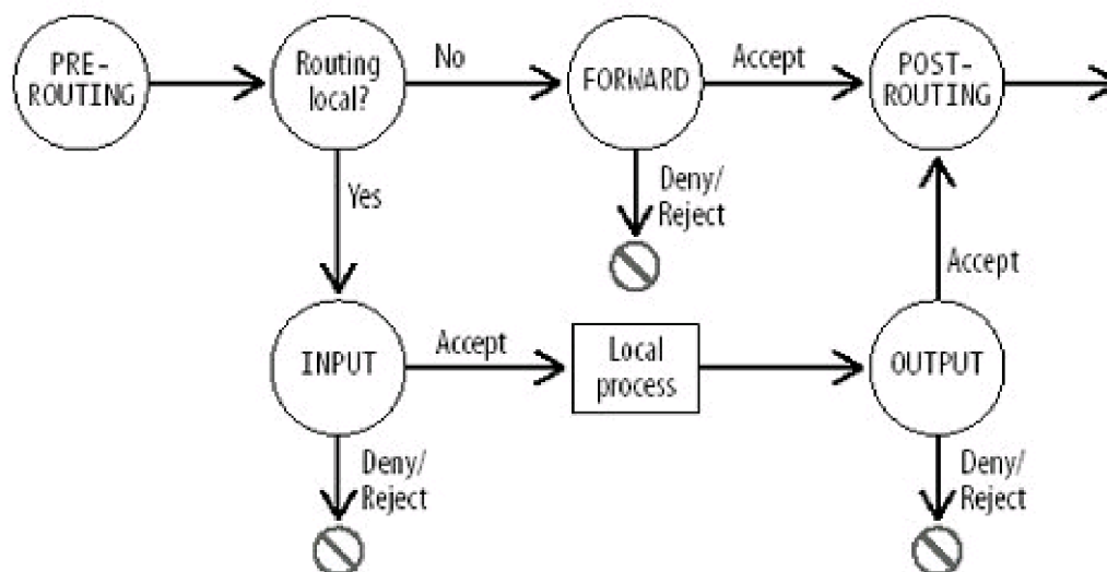
Figure 40-3. Chains and traffic flow in iptables
