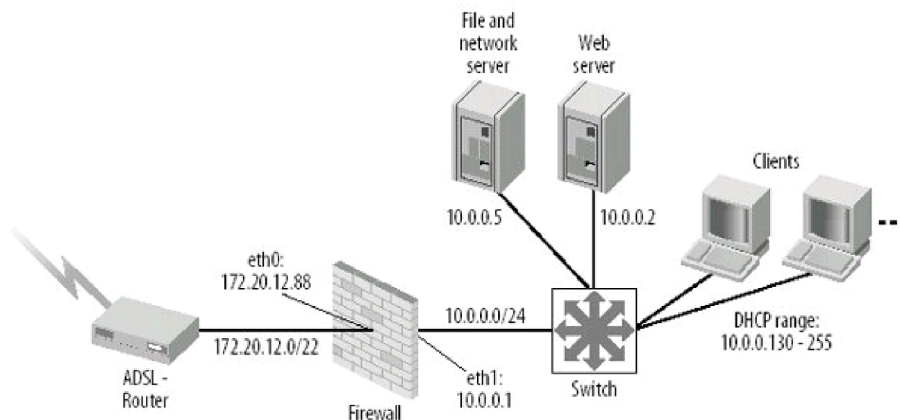
Figure 40-1. Network diagram for example network
