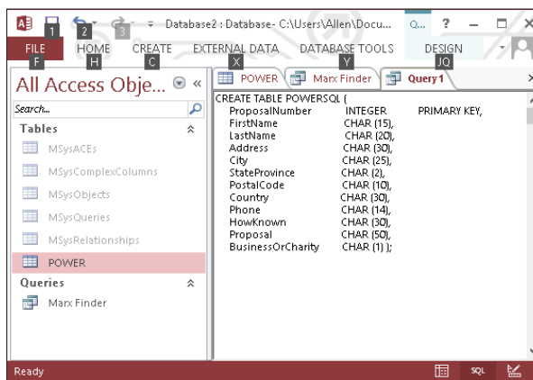
Figure 4-14: Data-definition query to create a table.
