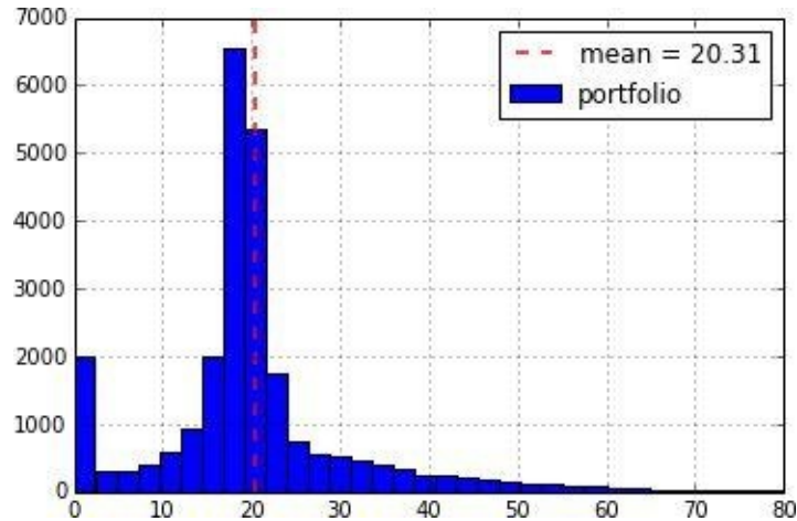
Figure 18-4. Portfolio frequency distribution of present values
