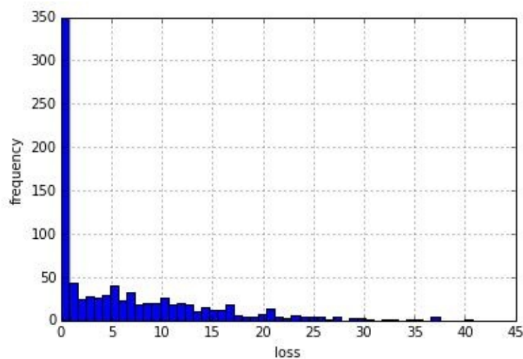
Figure 10-22. Losses due to risk-neutrally expected default (call option)
