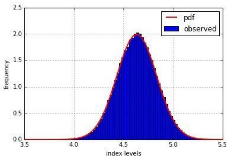
Figure 11-5. Histogram of log index levels and normal density function
