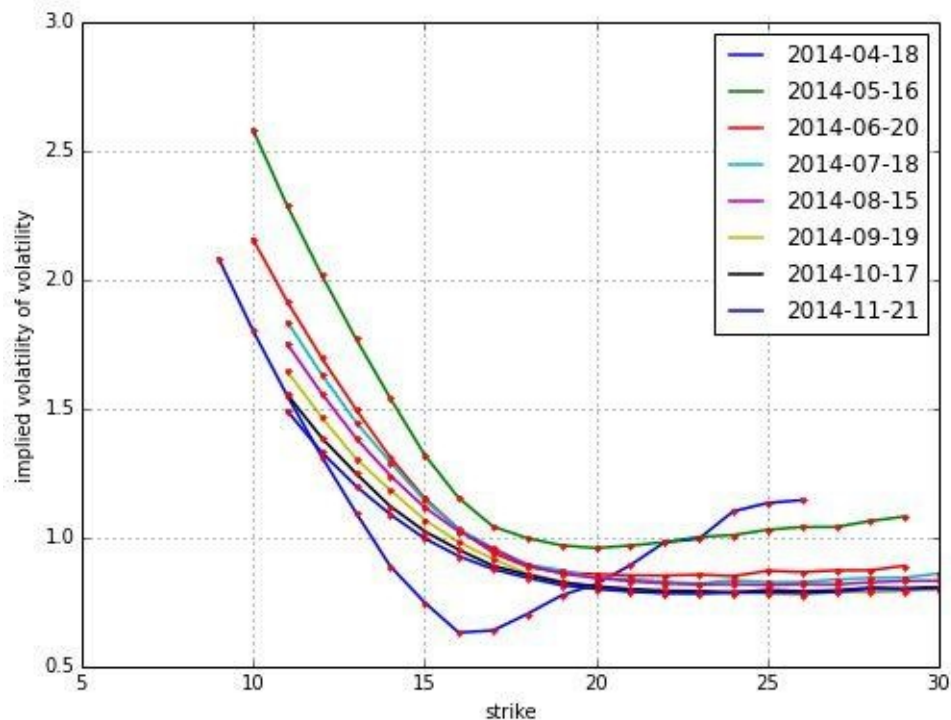
Figure 3-1. Implied volatilities (of volatility) for European call options on the VSTOXX on March 31, 2014
