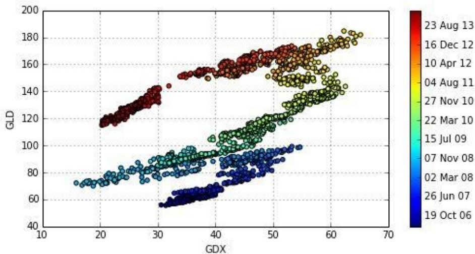
Figure 11-23. Scatter plot of prices for GLD and GDX
