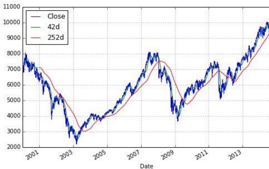
Figure 6-5. The DAX index and moving averages
