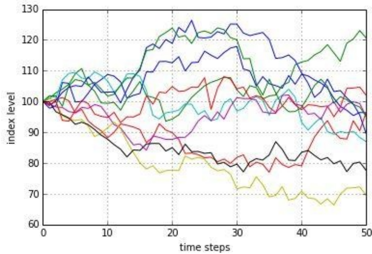
Figure 11-1. Ten simulated paths of geometric Brownian motion
