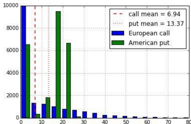
Figure 18-3. Portfolio frequency distribution of present values
