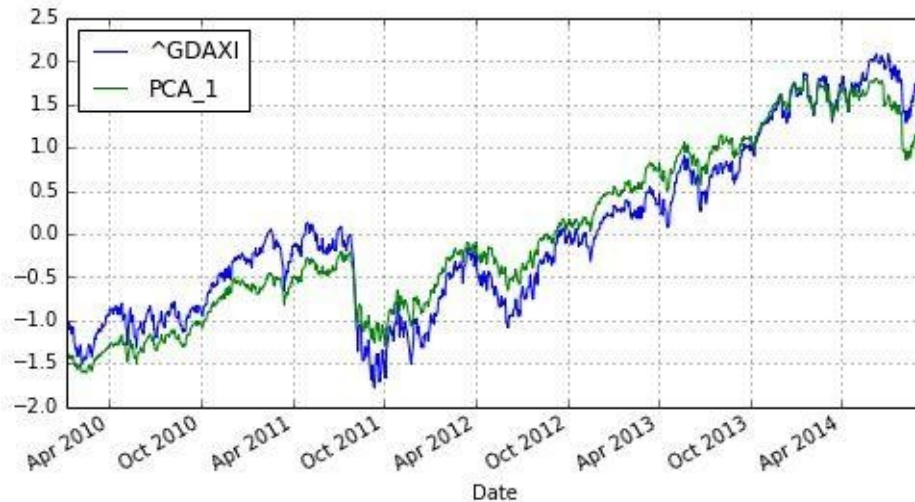
Figure 11-15. German DAX index and PCA index with one component
