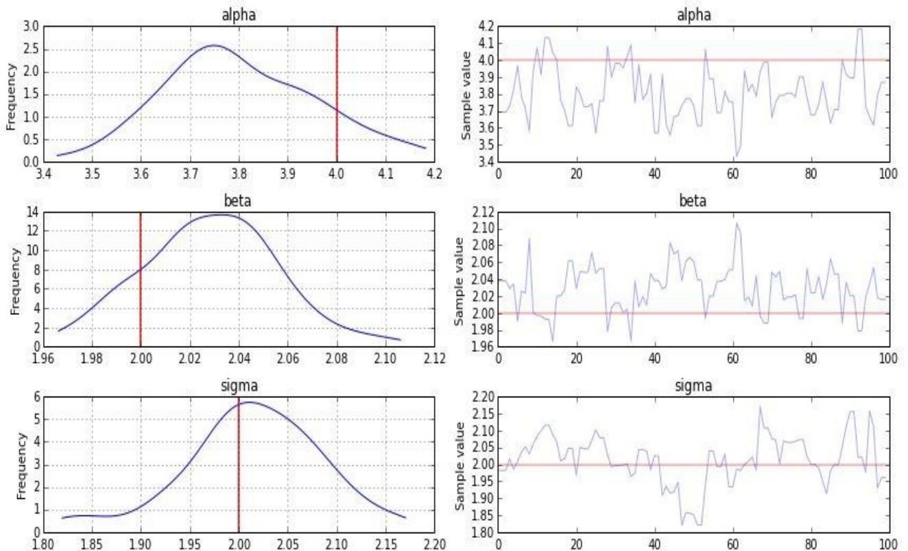
Figure 11-20. Trace plots for alpha, beta, and sigma
