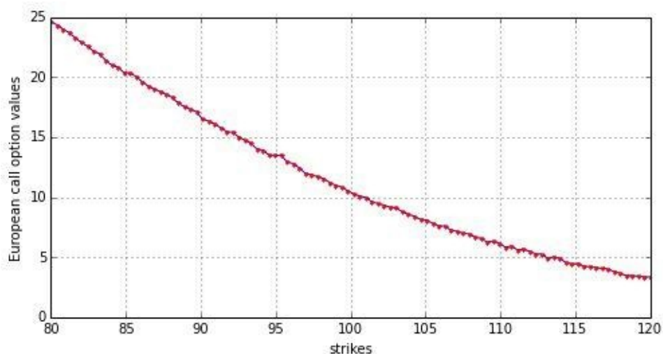
Figure 8-1. European call option values by Monte Carlo simulation
