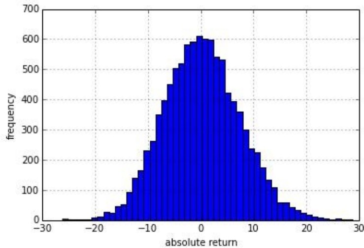
Figure 10-18. Absolute returns of geometric Brownian motion (30d)
