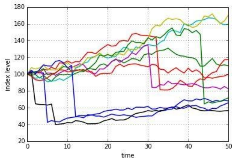
Figure 10-14. Simulated jump diffusion paths
