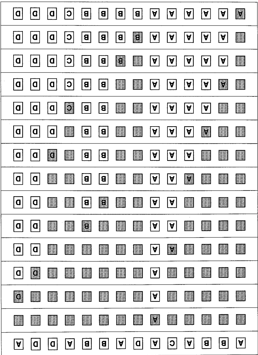
Figure 8.11 Distribution Counting.
