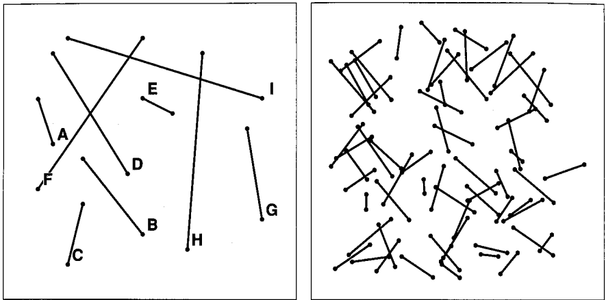
Figure 27.6 Two general line intersection problems.
