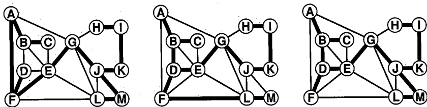
Figure 31.2 Minimum spanning trees.
