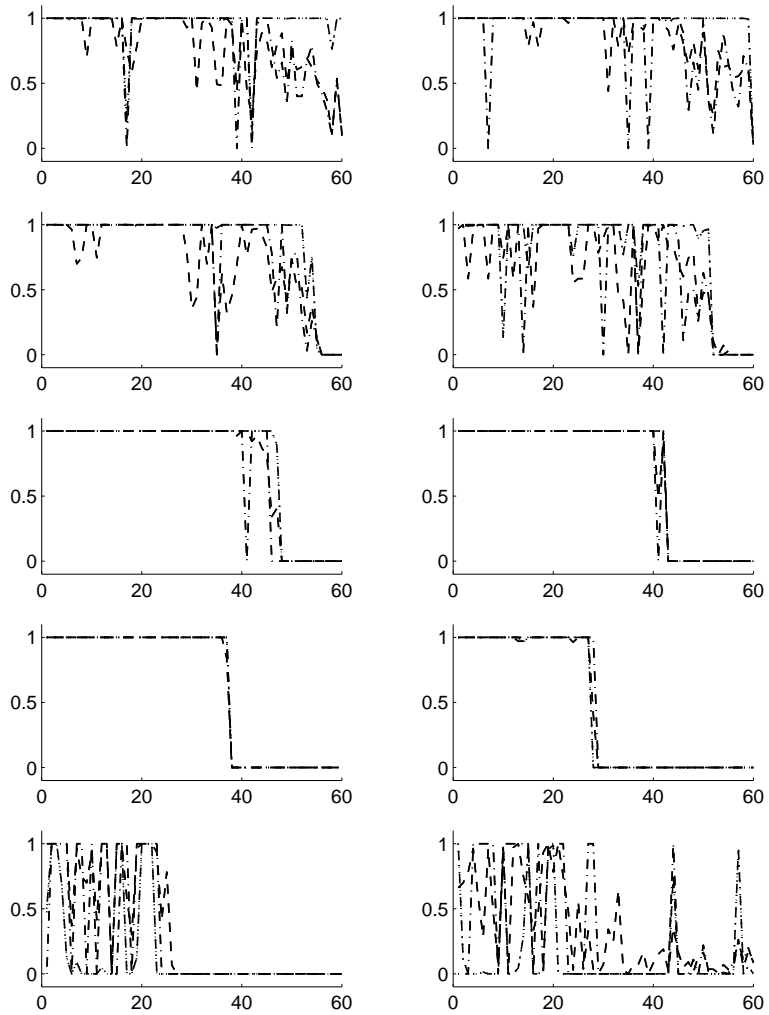
Figure 6.13: Posterior estimates of the probability of being in the free-flow state for the 4-5pm model on test sequence 2. Dotted lines represent exact/BK (which are indistinguishable at this resolution), dot-dash is PF with 100 particles, and dash-dash is PF with 1000 particles. Plots denotes locations 1 to 10 in left-right, top-bottom order. Notice how the change from free-flow to congested takes place earlier in the downstream locations.
