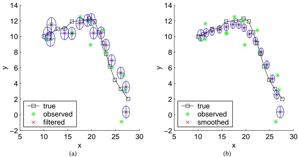
Figure 1.3: Results of inference for the the tracking problem in Section 1.3.1. (a) Filtering. (b) Smoothing. Boxes represent the true position, stars represent the observed position, crosses represented the estimated (mean) position, ellipses represent the uncertainty (covariance) in the position estimate. Notice that the smoothed covariances are smaller than the filtered covariances, except at t = T , as expected.
