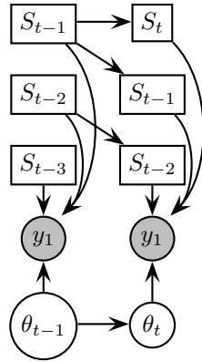
Figure 2.32: A DBN for blind deconvolution.
