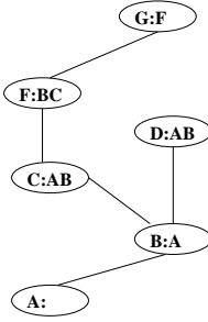
Figure B.8: An elimination tree derived from Figure B.6. The notation C : A, B means, when C was eliminated, \{A, B\} were the uneliminated neighbors.
