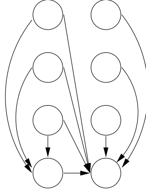
Figure 3.2: A worst case DBN from a complexity point of view, since we must create a clique which contains all nodes in both slices.
