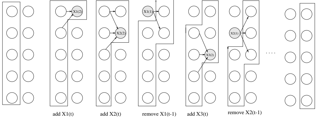
Figure 3.1: The frontier algorithm applied to a coupled HMM with 5 chains (see Figure 2.11); observed leaves (i.e., y_{1:T} ) are omitted for clarity. Nodes inside the box are in the frontier. The node being operated on is shown shaded; only connections with its parents and children are shown; other arcs are omitted for clarity. See text for details.
