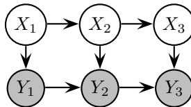
Figure 2.5: An auto-regressive HMM.
