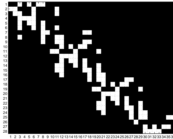
Figure 3.11: A representation of the cliques in the constrained Mildew jtree (Figure 3.9). Each row represents a clique, each column represents a DBN variable. The repetitive structure in the middle of the jtree is evident. For example, rows 17 and 25 are isomorphic, because their “bit pattern” is the same (101100011), and is exactly 9 columns apart. (The bit pattern refers to the 0s and 1s, which is a way of representing which DBN nodes belong to each clique set.)
